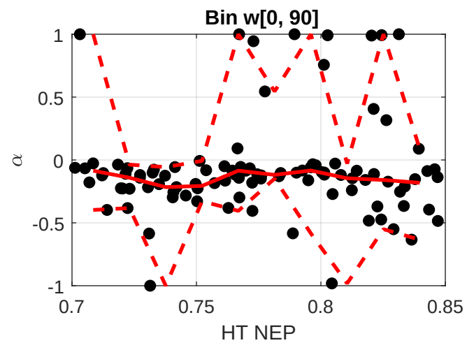
rel h um|temp: H&T parameter stability by threshold
